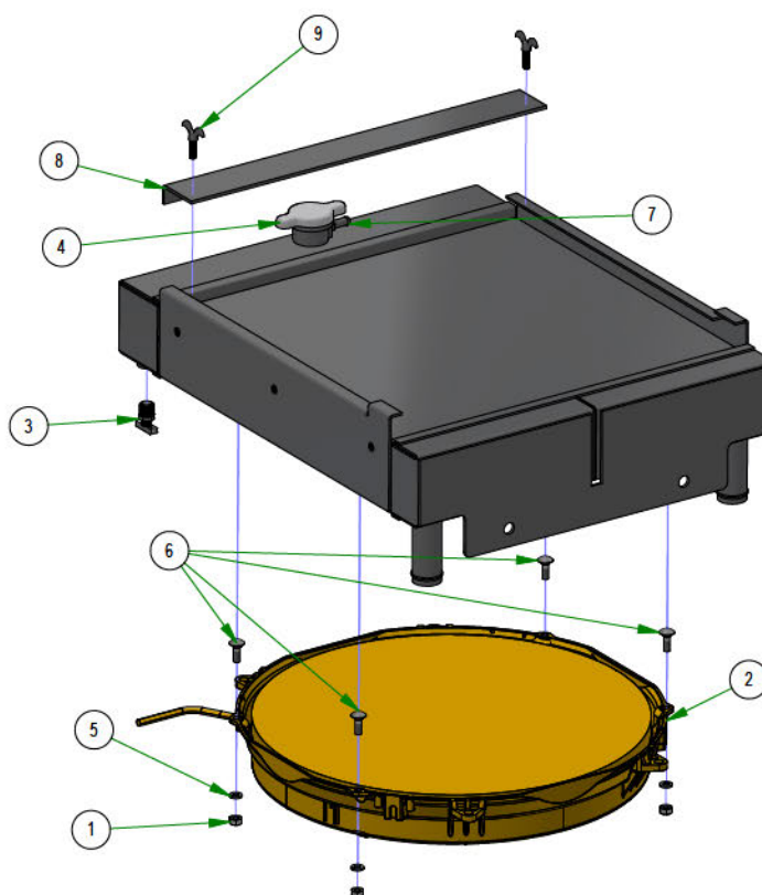
061-5001-00 RADIATOR ASSEMBLY
