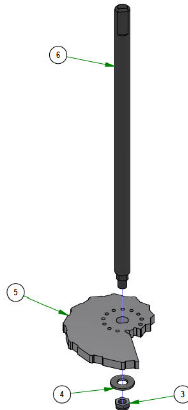
028-0015-19 DECK HEIGHT CAM ASSEMBLY
