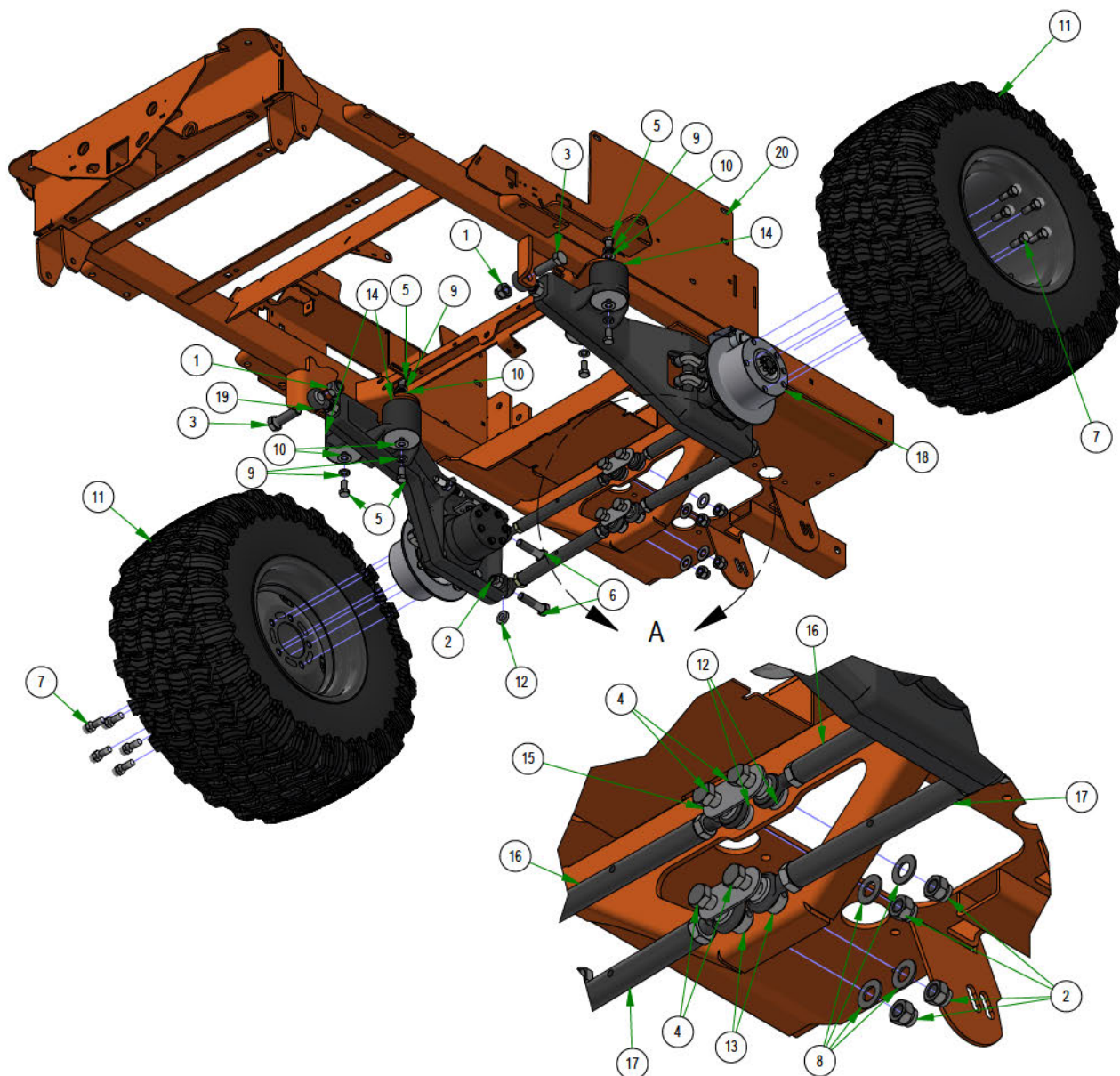
DETAIL A
